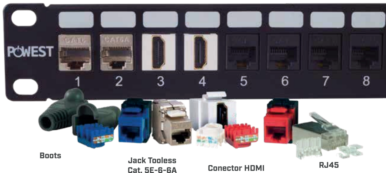
Patch Panel
